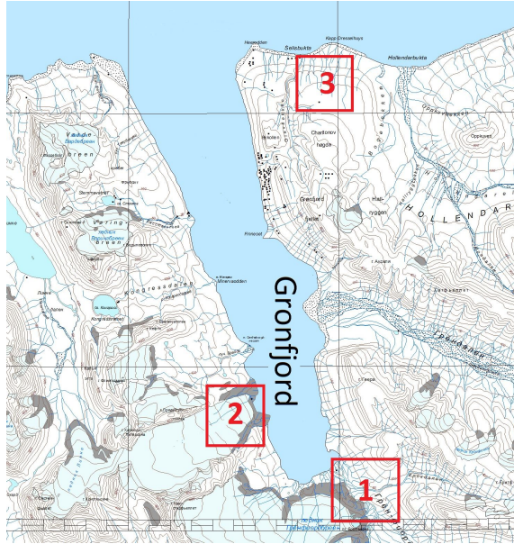
Fig. 1. The map of study area (key plots). 1 – Grondasselva river; 2 – Aldegonda river; 3 – sea terrace in surroundings of Barentsburg aerodrome.
