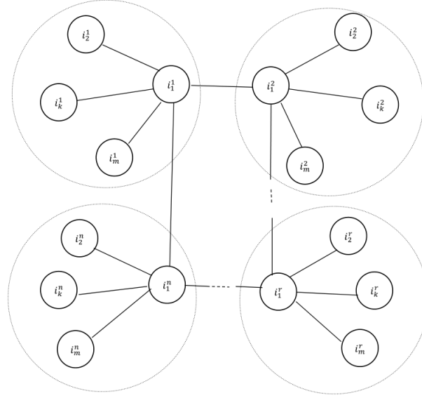
Fig. 1. The connections of the Multi-star model
