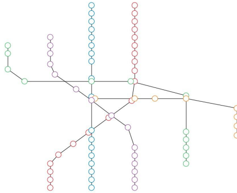
Fig. 5. St. Petersburg subway graph
