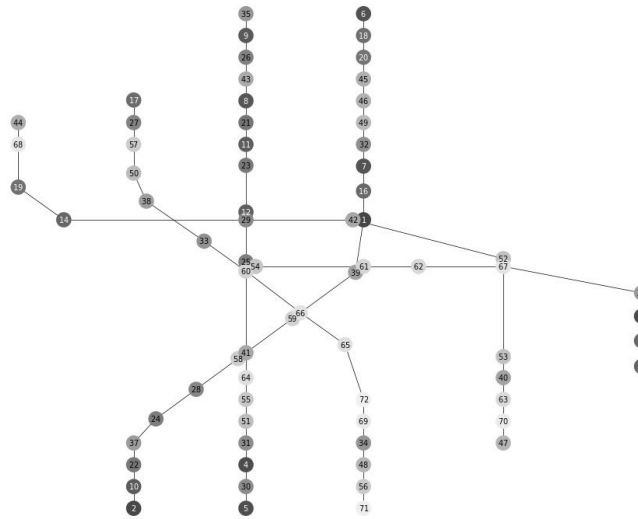
Fig. 7. St.Petersburg subway graph with weighted edges and vertices
