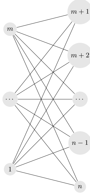
Fig. 4. Bipartite graph K_{m,n-m}
