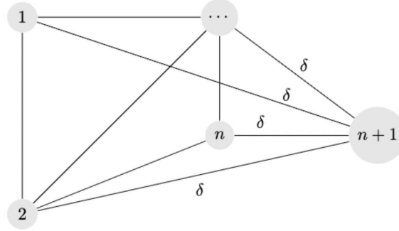
Fig. 1. Graph G' with an artificially added vertex v_{n+1}
