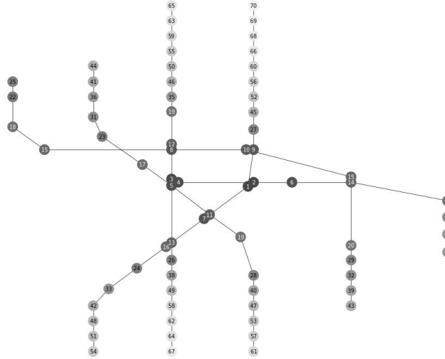
Fig. 6. St.Petersburg subway graph with weighted edges
