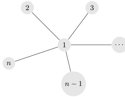
Fig. 3. Star graph S_n
