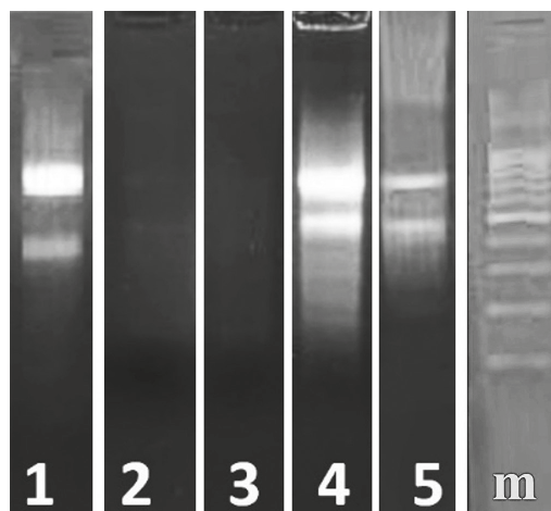
Fig. 2. Agarose gel electrophoresis of total RNA isolated from apple seeds of cv. Golden Delicious using various methods. Lane 1 — presented method; lane 2 — presented method without SiO 2 ; lane 3 — Quick-RNA MiniPrep; lane 4 — CTAB-method; lane 5 — presented method; lane m — marker (100–1000 bp); using denaturing RNA samples for electrophoresis in TAE agarose gel.
