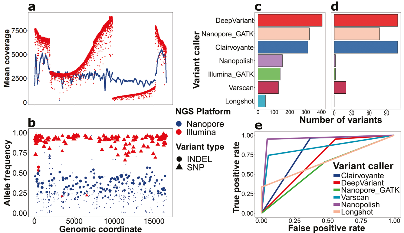
Fig. 1. The comparative analysis of different sequencing platforms and variant calling pipelines. (a) Mean per-site sequencing depth across the mitochondrial genome. Red color denotes the Illumina data; blue color refers to the ONT long reads. (b) Shown is the distribution of the variants obtained. Color code is identical to (a) ; circles stand for INDELs, and triangles represent SNPs; the size of the points is proportional to the number of programs reported the variant. (c) The sum of raw calls for each pipeline. (d) Cumulative numbers of variants uniquely called with each instrument. (e) ROC (receiver operating characteristic) curves of false-positive and false-negative rates for callers applied at the Nanopore data comparing to the Illumina-based calls.
